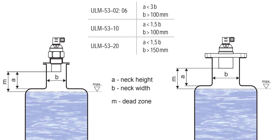
Possible installation through the neck
