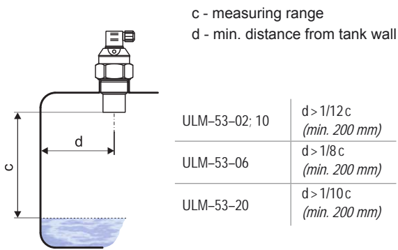
Installation distance from the tank wall
